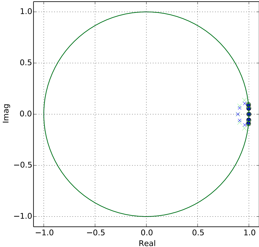
NTF Poles and Zeros
