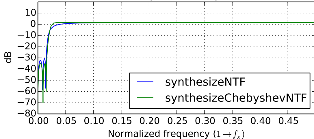
NTF Magnitude Response
