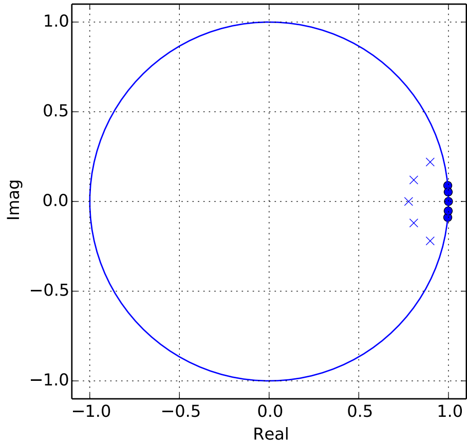
Poles and Zeros
