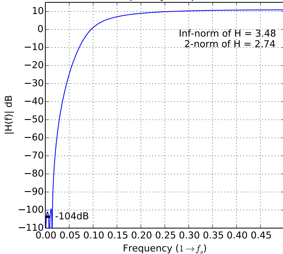
Frequency Response
